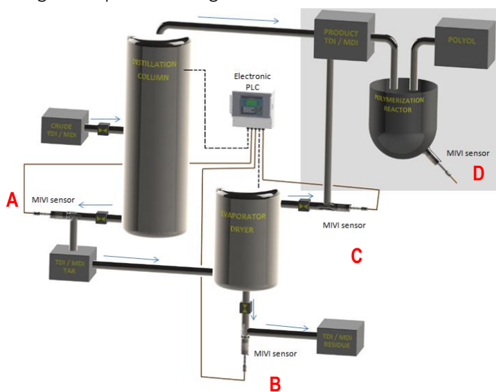
MDI/TDI global operation diagram for MIVI sensors
